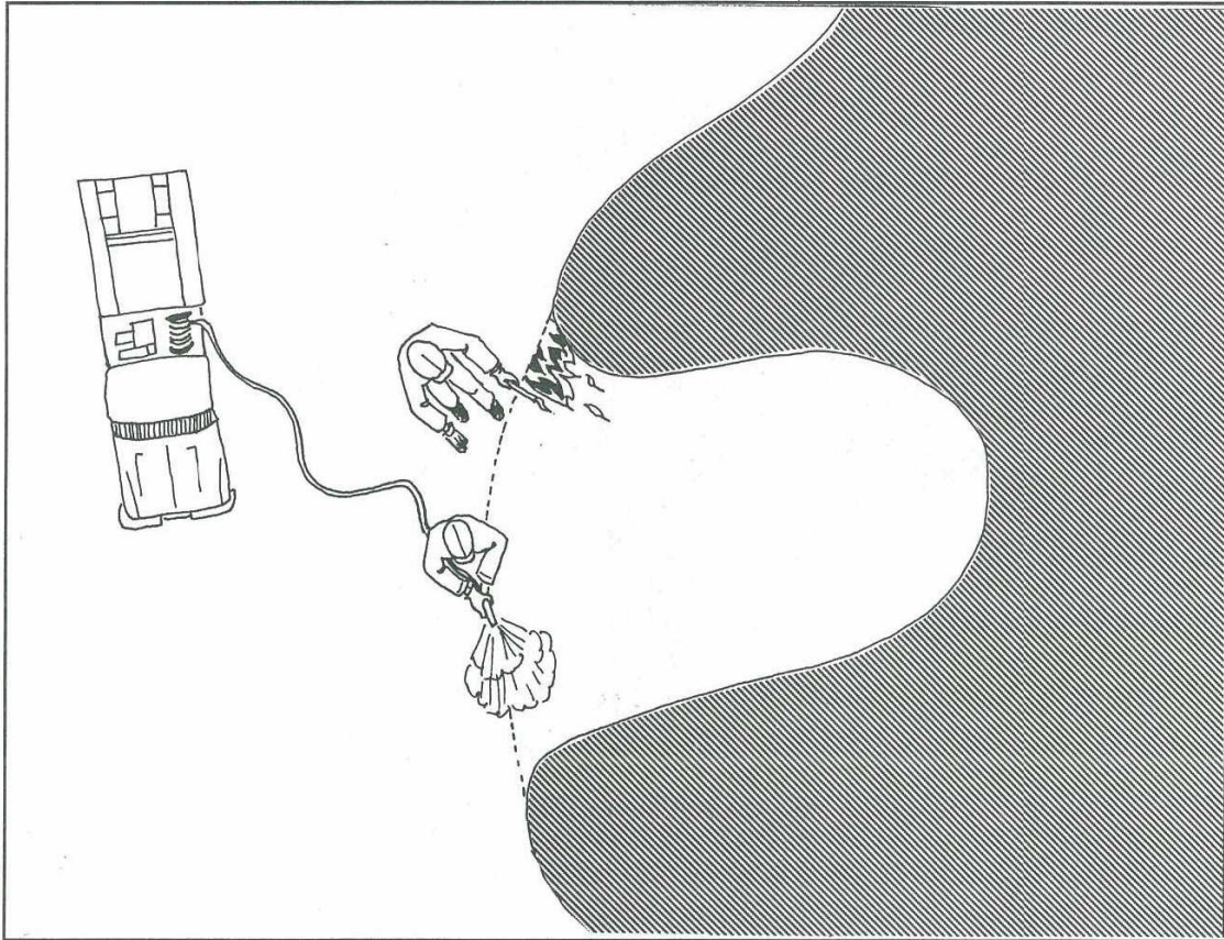
Figure 18 – Parallel Attack With Wetline and Burn Out
