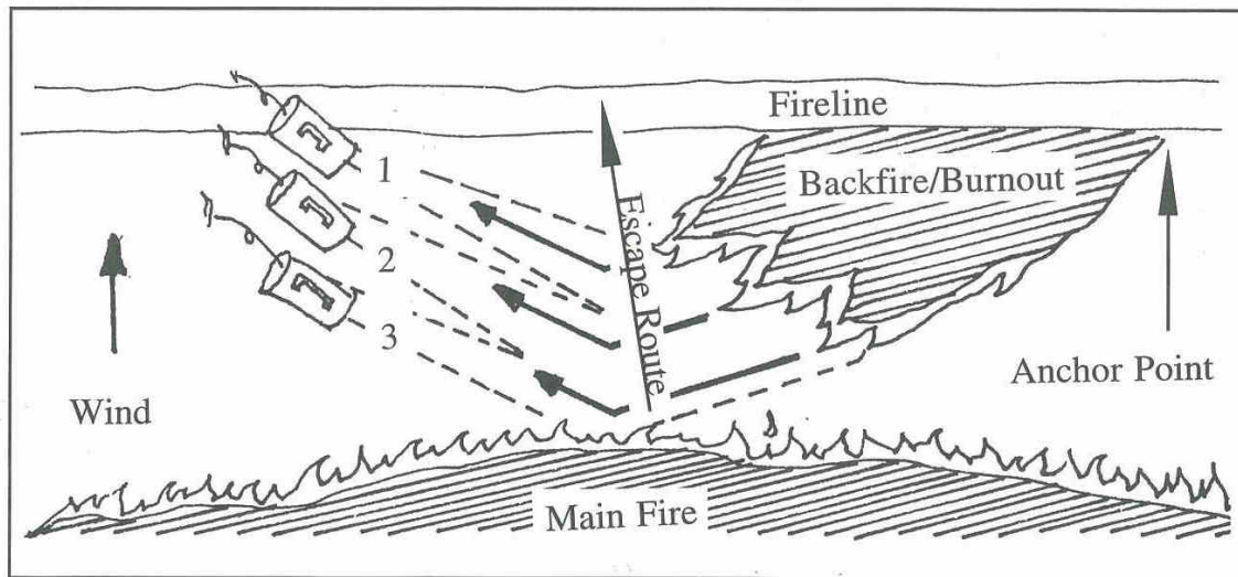
Figure 14 – Blowhole Firing Backfiring Against the Wind (1-2-3 Organization)
