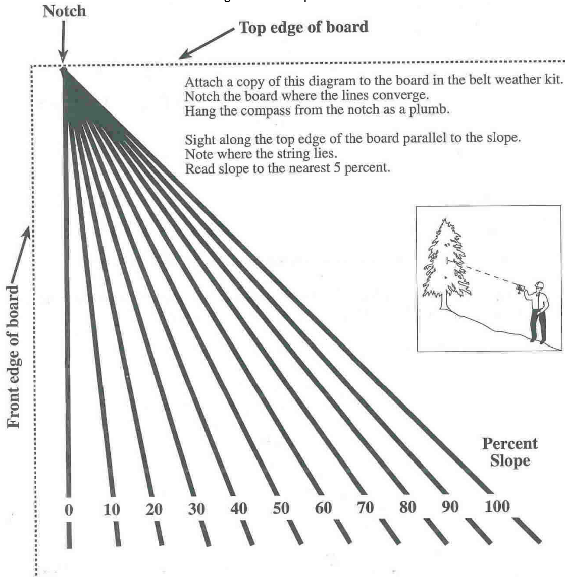
Figure 3 – Slope Meter
