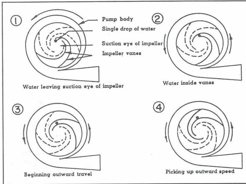
Figure 1 – Centrifugal Pump
