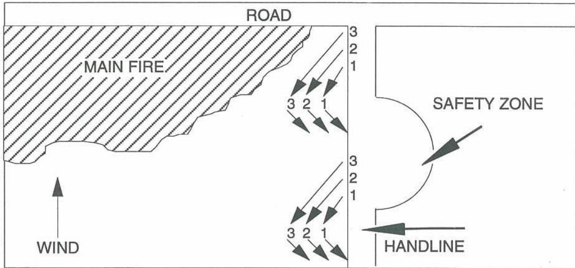
Figure 15 – Blowhole Firing (Backfiring/Burning Out on Flanks)
