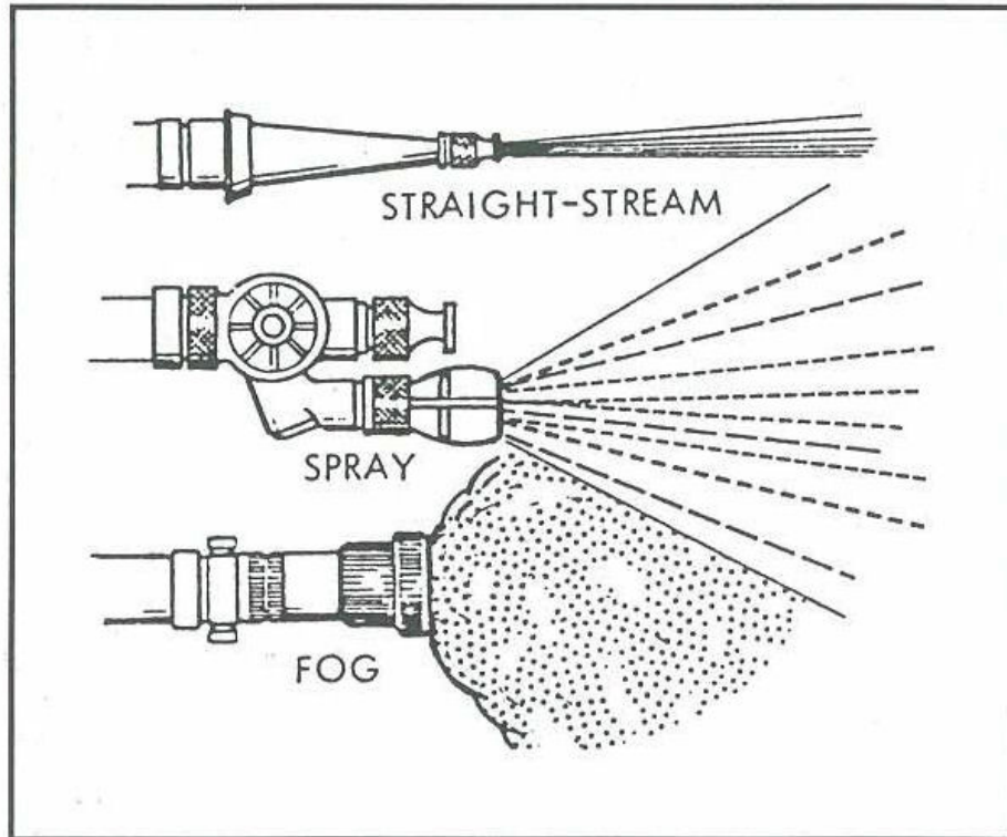
Figure 15 – Nozzle Types
