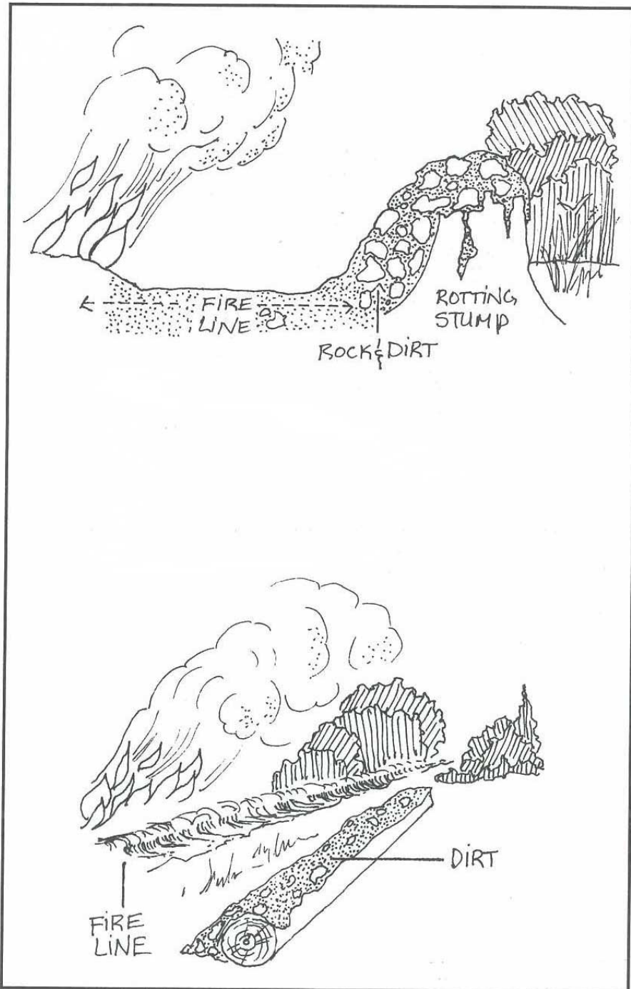
Figure 18 – Protection of Stumps and Logs Outside Fireline
